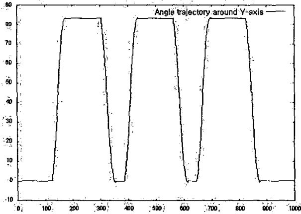
Fig. 11. Angle trajectory around Y-axis with compensation algorithms(deg).
