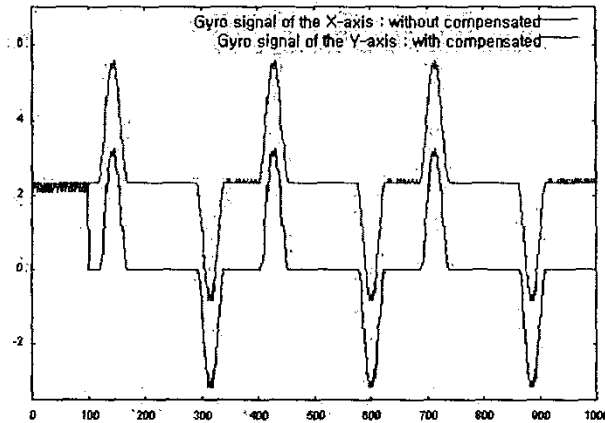
Fig. 13. Gyro output signal of Y-axis(deg/sec).
