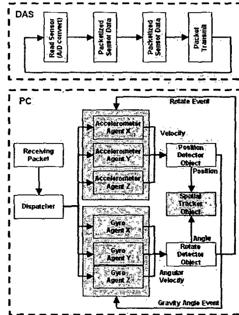
Fig. 2. Spatial tracking system software structure.
