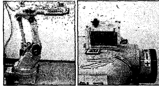
Fig. 6. Experiment Setup to Evaluate the Spatial Tracker System.
