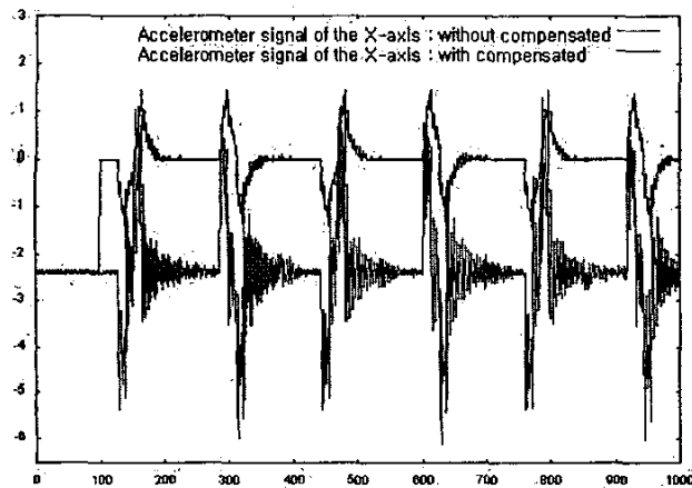
Fig. 7. Accelerometer output signal of X-axis(m/sec 2 ).
