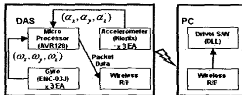
Fig. 1. Spatial tracker system block diagram.
