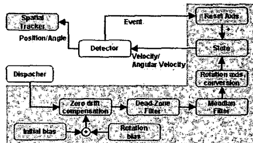
Fig. 4. Signal processing flow in the Sensor Agent
