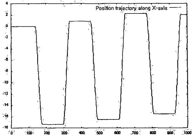
Fig. 8. Position trajectory along X-axis with compensation algorithms(cm).
