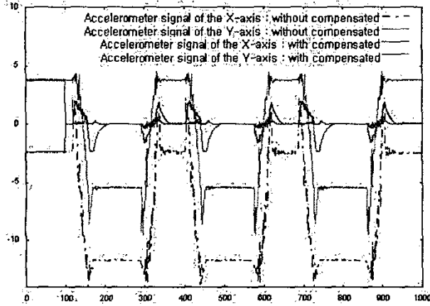
Fig. 12. Accelerometer output signals of X- and Z-axes(m/sec 2 ).
